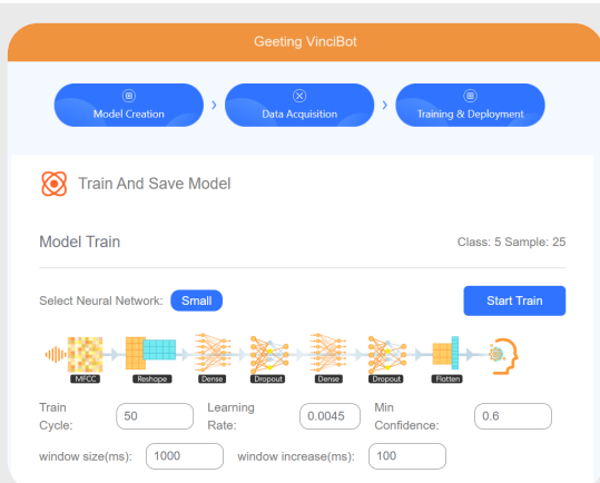
Step 3: Train and deploy the model
